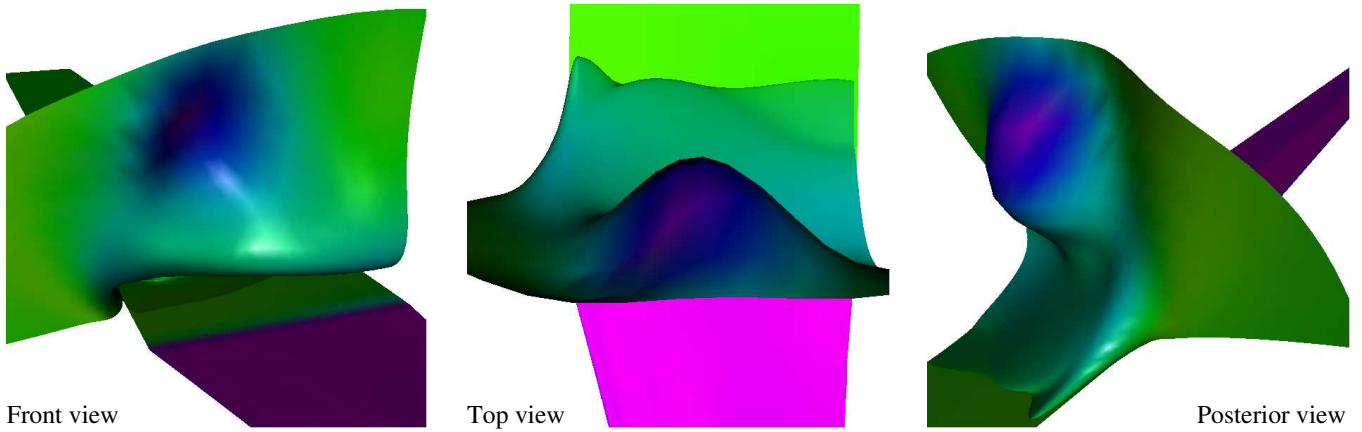
Color Plate 2: Delta wing flow strain rate deviator → negative surface normal
