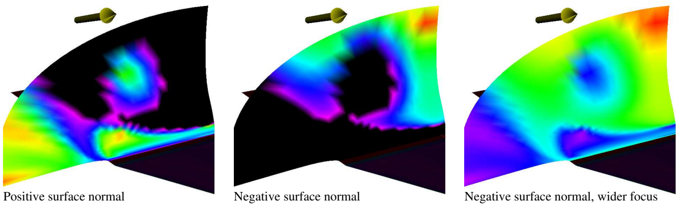
Color Plate 3: Delta wing flow strain rate deviator → directional visualization
