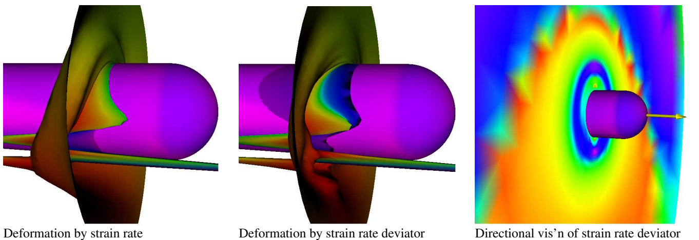
Color Plate 5: Cylinder with hemispherical head → grid slice
