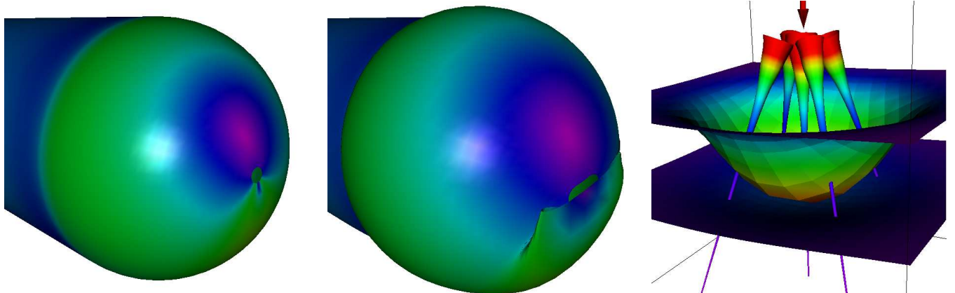
Color Plate 4: Cylinder with hemispherical cap → deformation of cap
